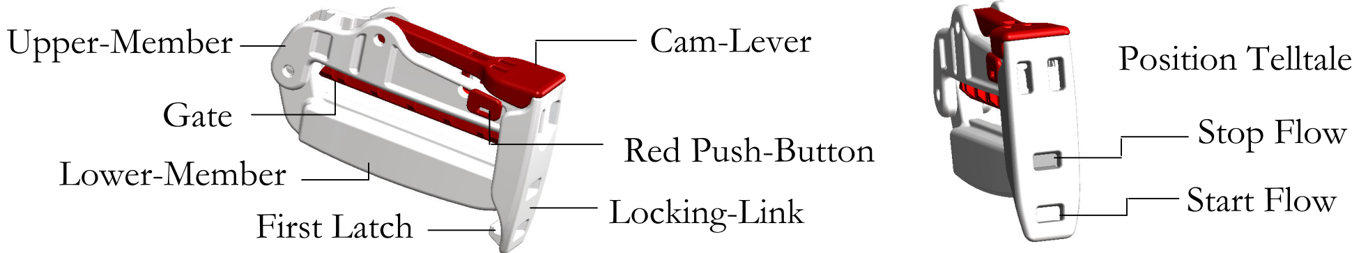
HWC Stop Flow with Cable-Tie Lockout-1
